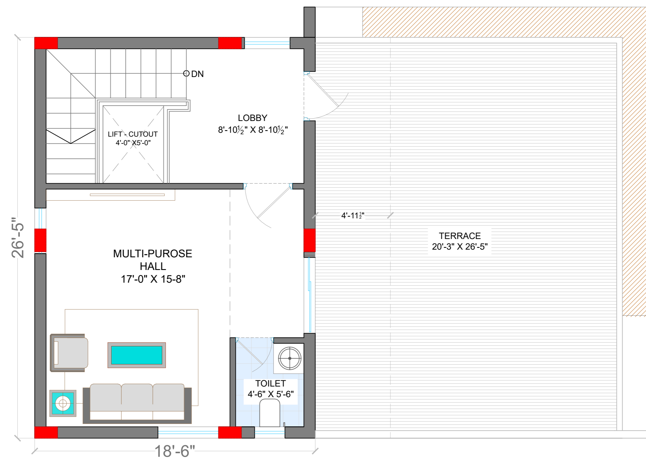
TERRACE FLOOR PLAN AREA - 619 sq ft
