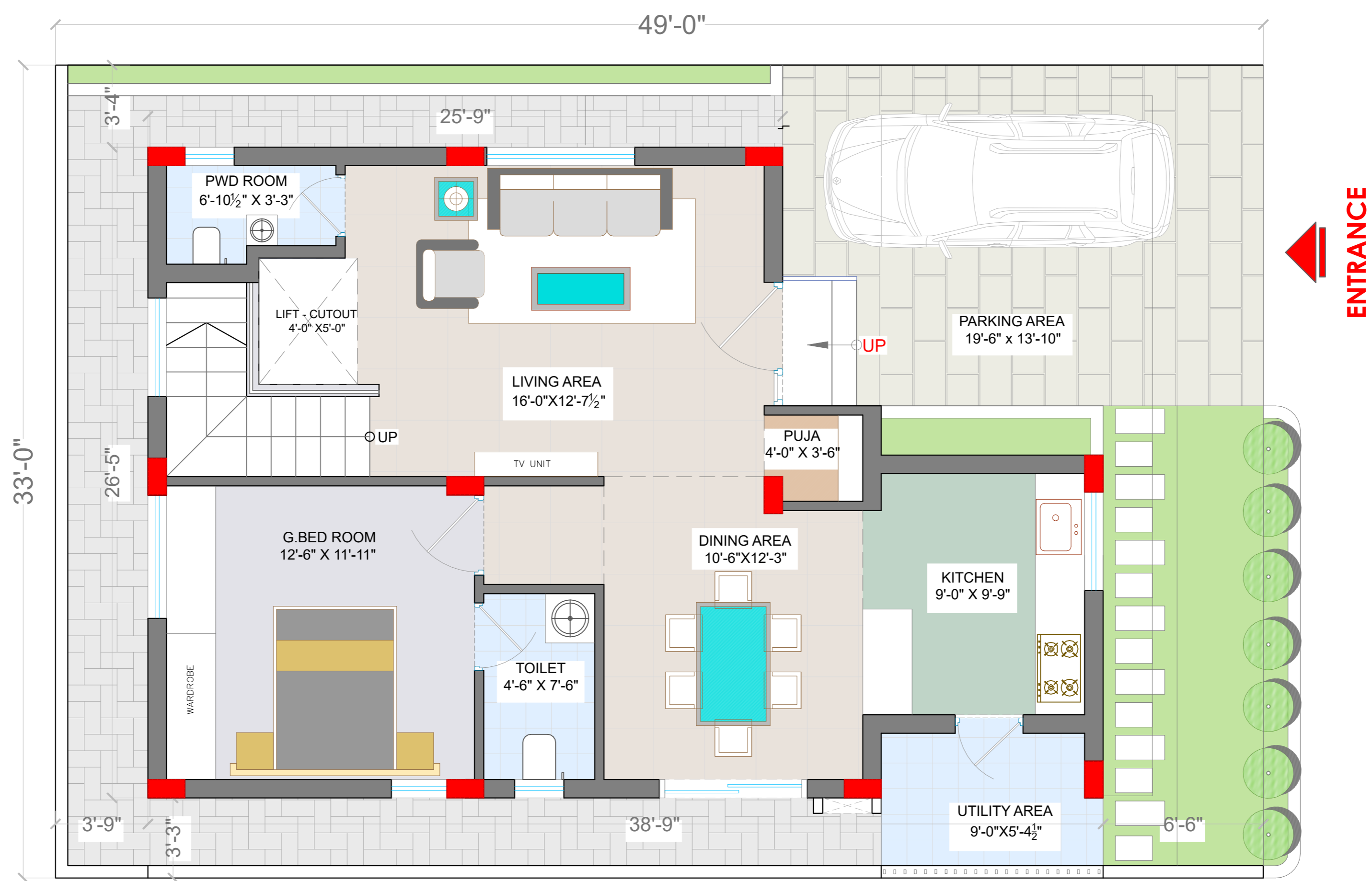
GROUND FLOOR PLAN FLOOR AREA - 1024 sq ft
