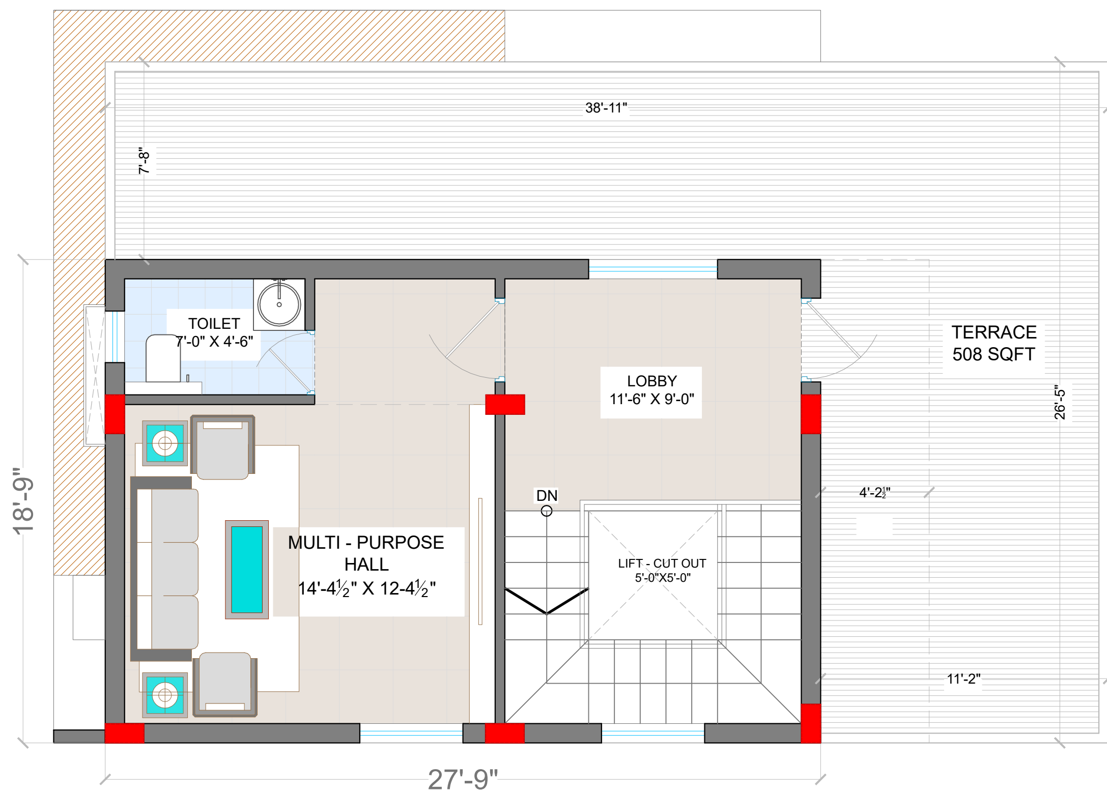
TERRACE FLOOR PLAN FLOOR AREA - 599 sq ft
