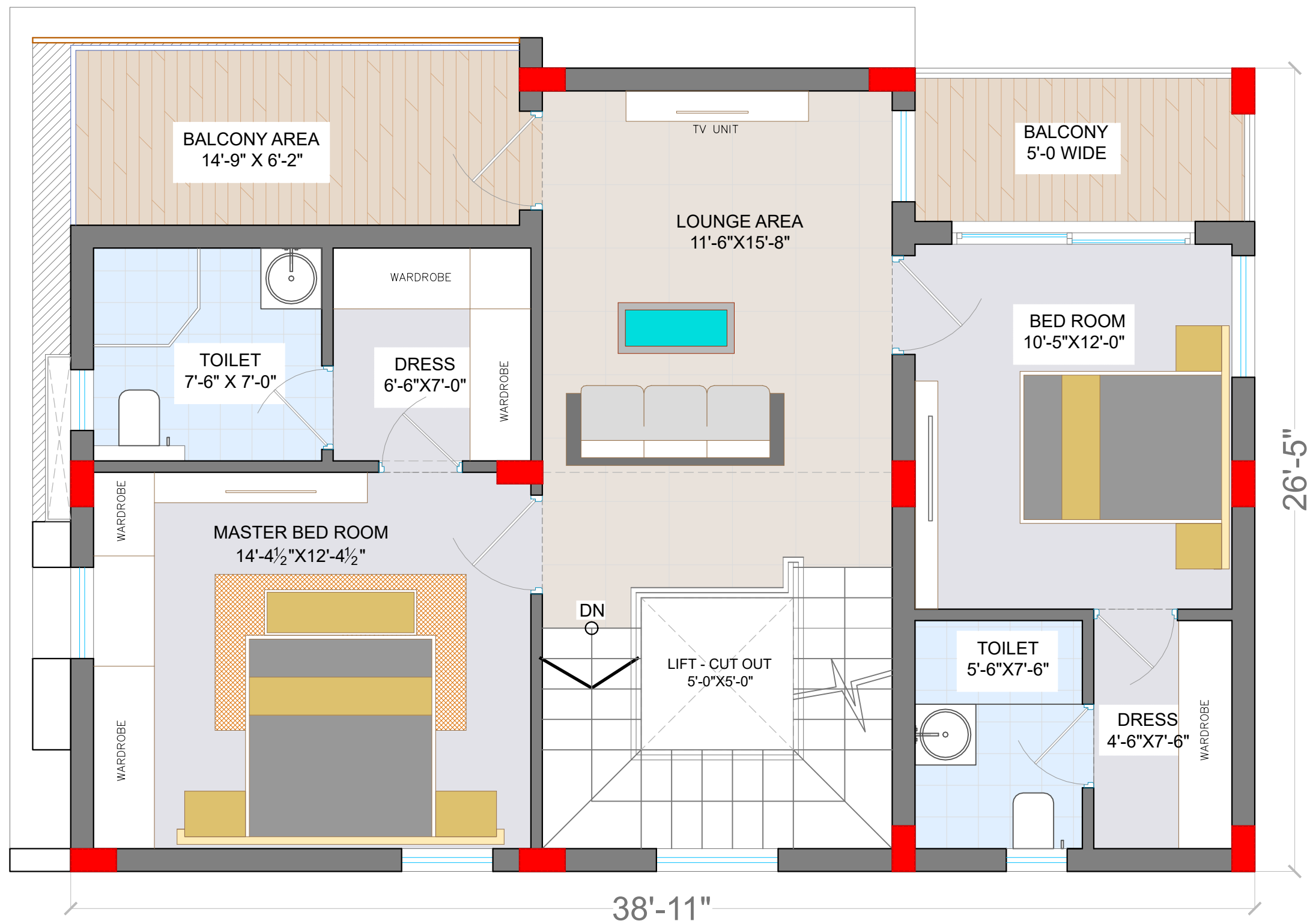
FIRST FLOOR PLAN FLOOR AREA -1,073 sq ft
