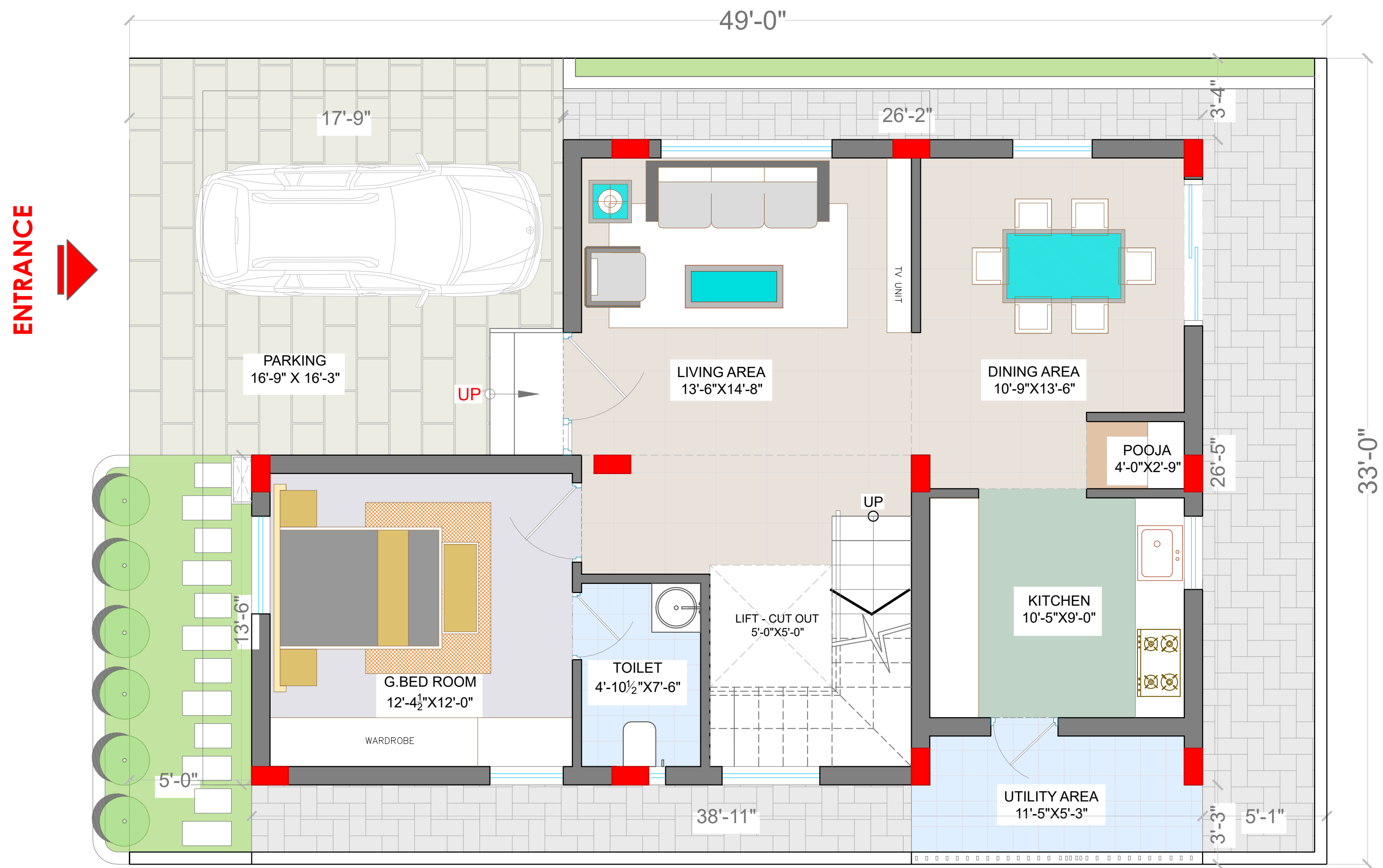
GROUND FLOOR PLAN FLOOR AREA - 1028 sq ft
