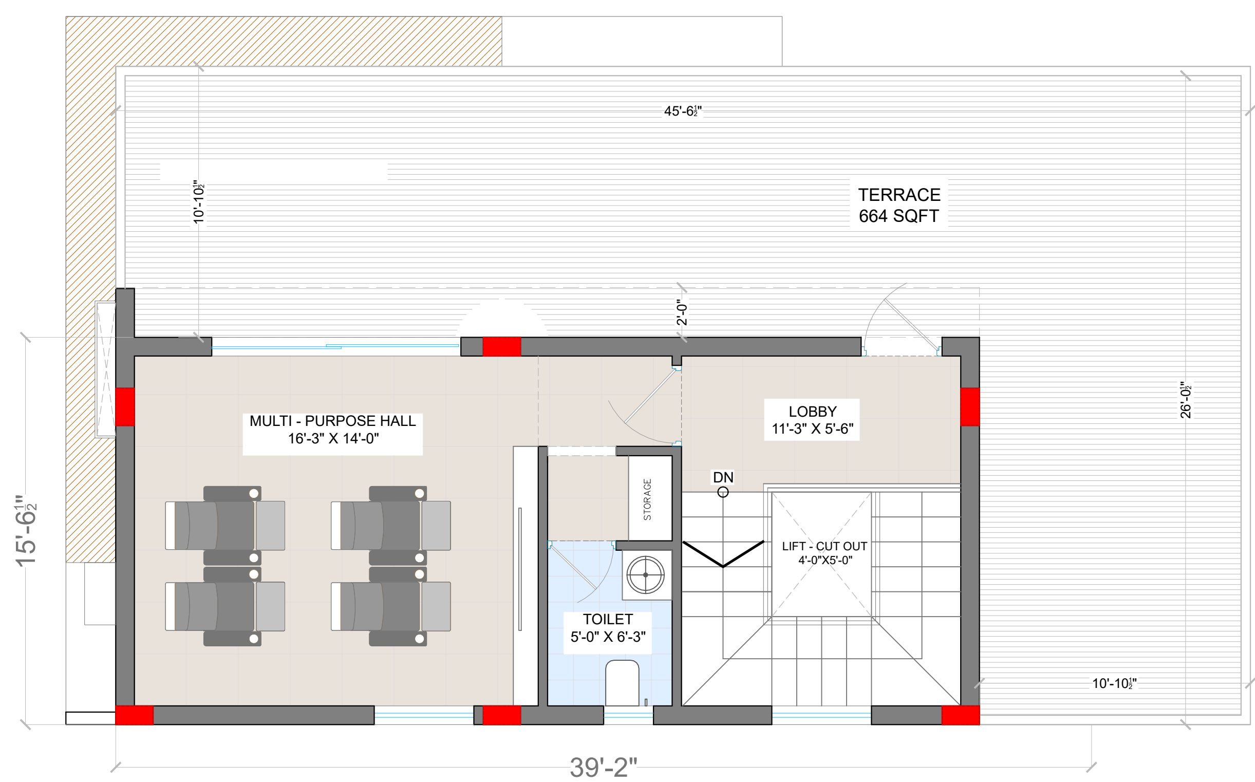
TERRACE FLOOR PLAN FLOOR AREA - 608 sq ft
