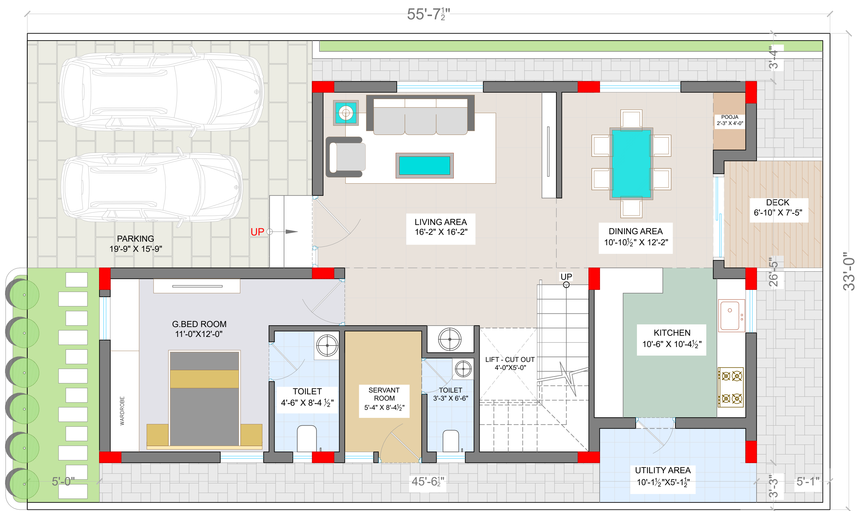
GROUND FLOOR PLAN FLOOR AREA - 1204 sq ft
