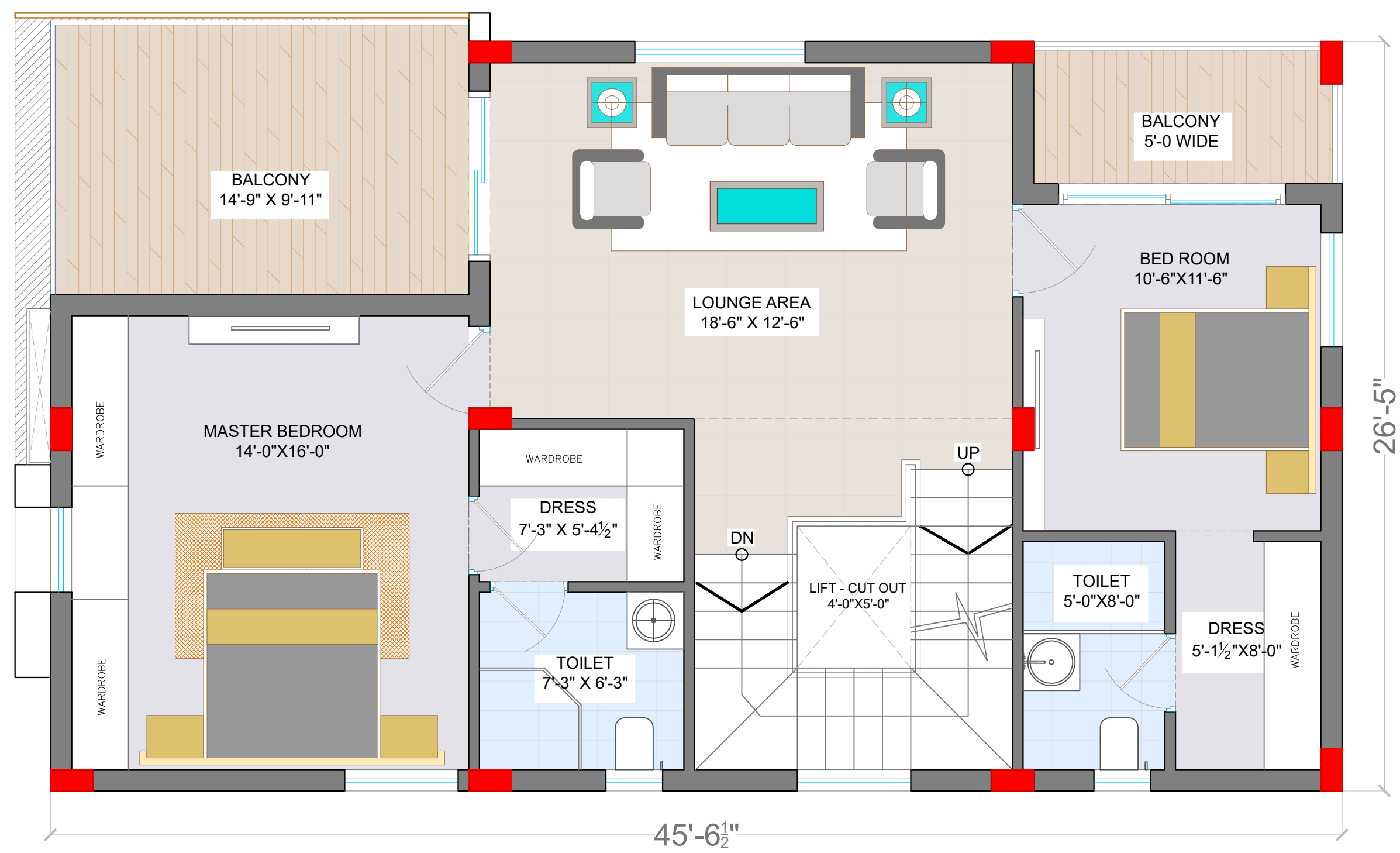
FIRST FLOOR PLAN FLOOR AREA - 1,248 sq ft
